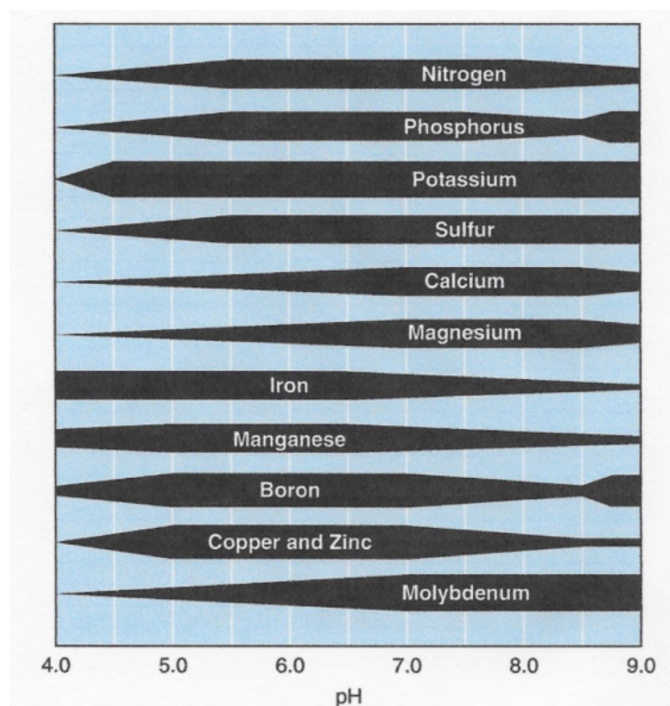
Figure 7. Nutrient availability chart by soil pH.
